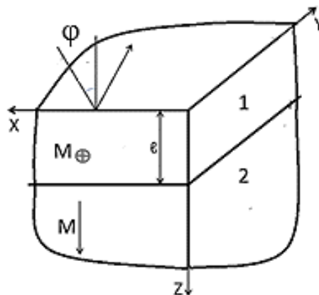
Fig 1. Schematic representation of the geometry of light reflection from a two-layer structure
