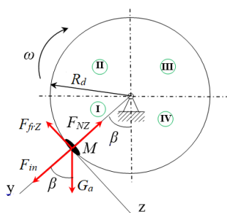
Figure: 3. Diagram of the acting forces along the YZ plane on a part of the paddy embankment
